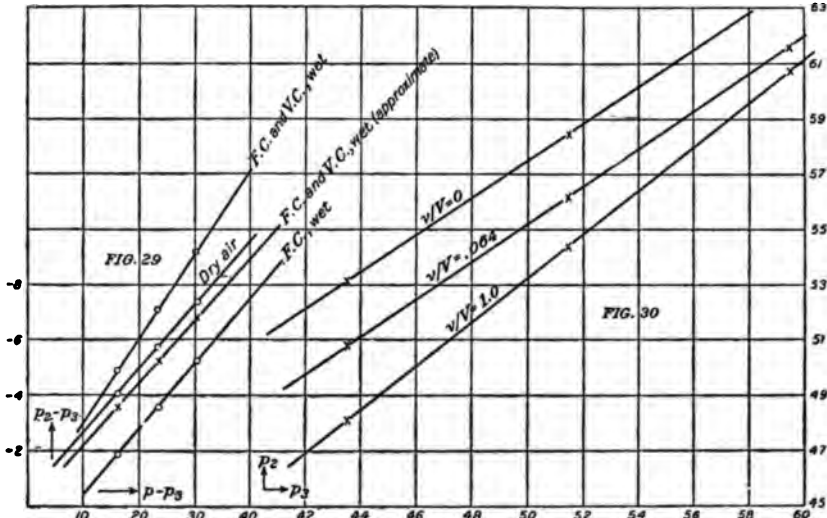
FIG. 29.—Corrections ( p_2 - p_3 ) for \delta p = p - p_3 . Table 20. FIG. 30.—Isothermal pressure p_2 in the isolated fog chamber for different isothermal pressures p_3 of the communicating fog chambers and for different volume ratios ( v/V ). Table 19.
